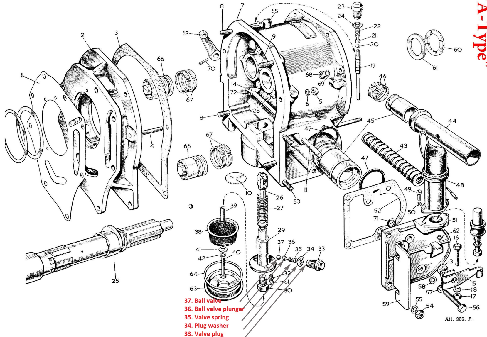
Fig. G.3. Components of overdrive front casing.
