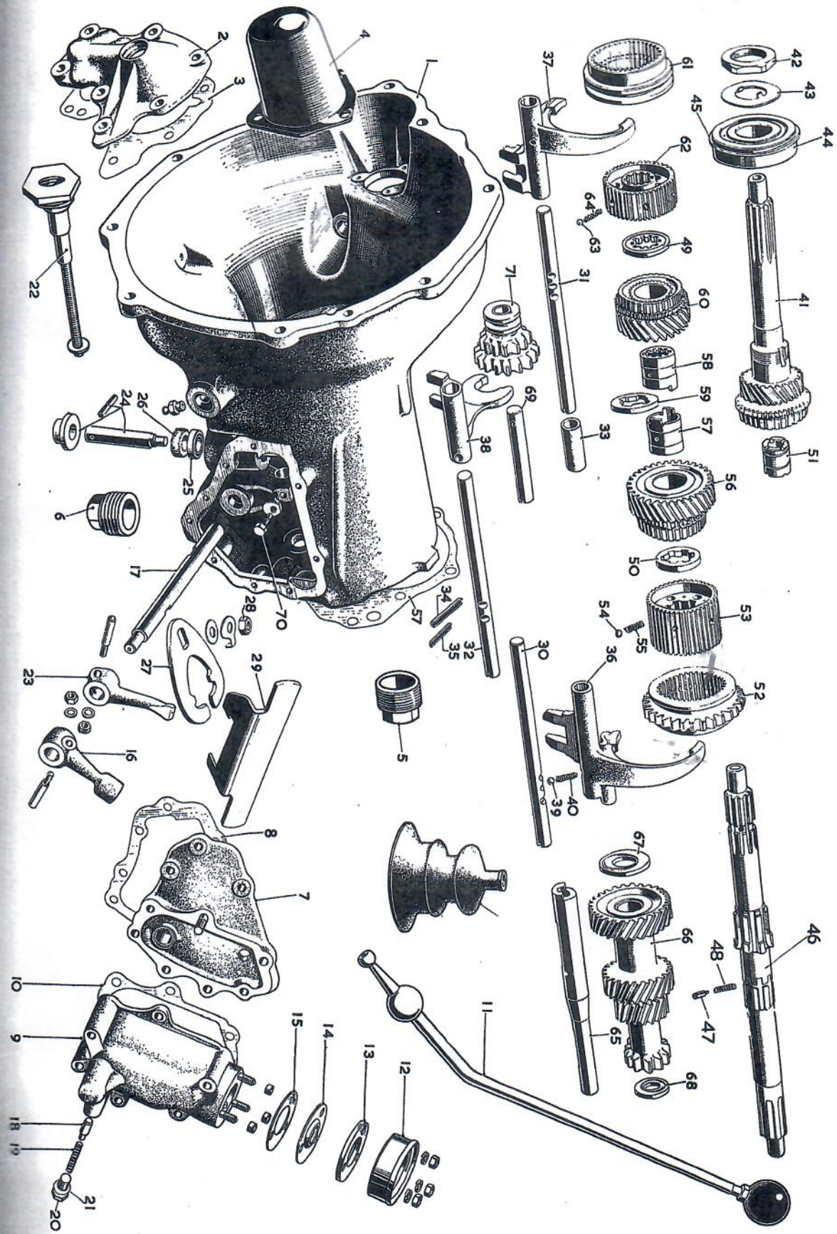
GEARBOX—PLATE B
