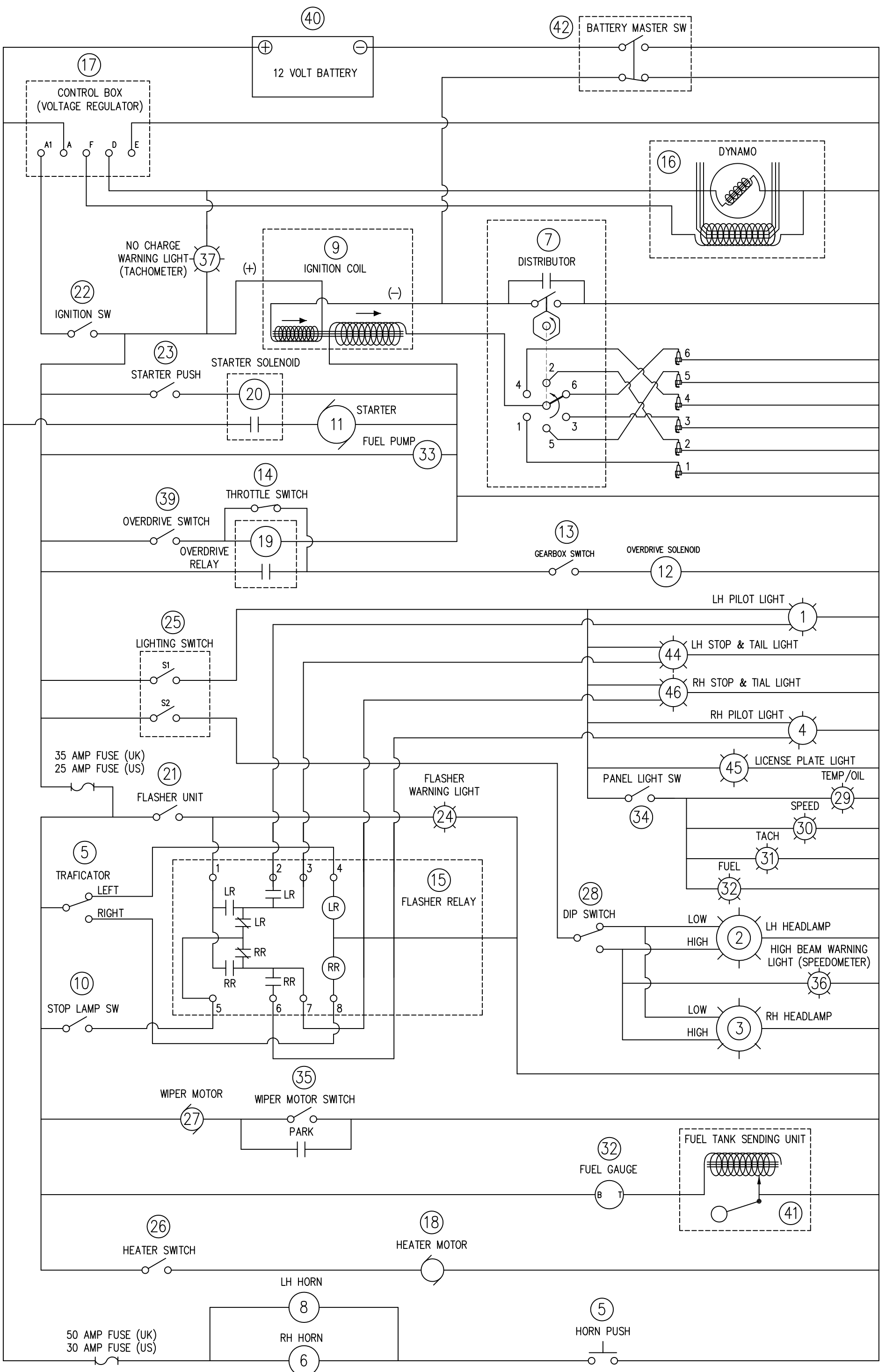
ELECTRICAL SYSTEM LOGIC (LADDER) DIAGRAM FOR AUSTIN HEALEY 3000 MKI BN7 AND BT7 ADAPTED FROM WIRING DIAGRAM ON PAGES 172 & 173 OF HAYNES OWNER'S WORKSHOP MANUAL COPYRIGHT 1974 (ISBN 0 900550 49 X)
