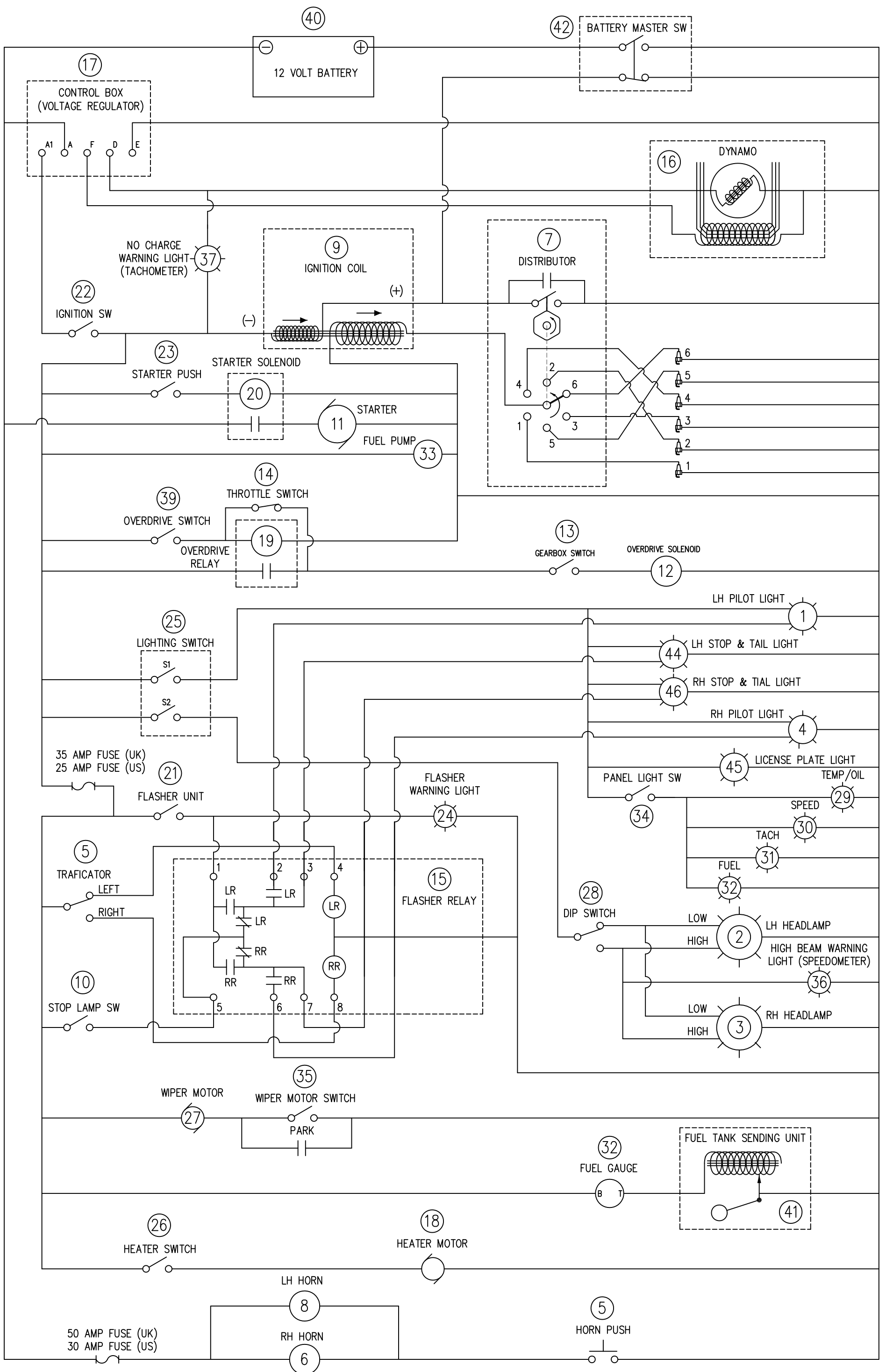
DIAGRAM FOR BN4 BN6 BN7 BT7 AND BJ7 CARS WITH STARTER PUSH AND OLD STYLE DASH EARLY BJ8 CARS WERE FITTED WITH A COMBINATION IGNITION AND STARTER SWITCH LATER BJ8 CARS WERE FITTED WITH SEPARATE TAIL/STOP AND DIRECTIONAL LIGHTS AND THE FLASHER RELAY WAS DELETED
